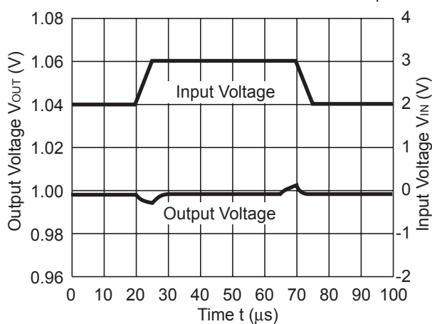
R1161x26xx (ECO=H)
