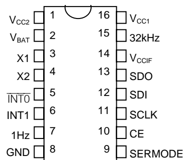
DIP (300 mils)
