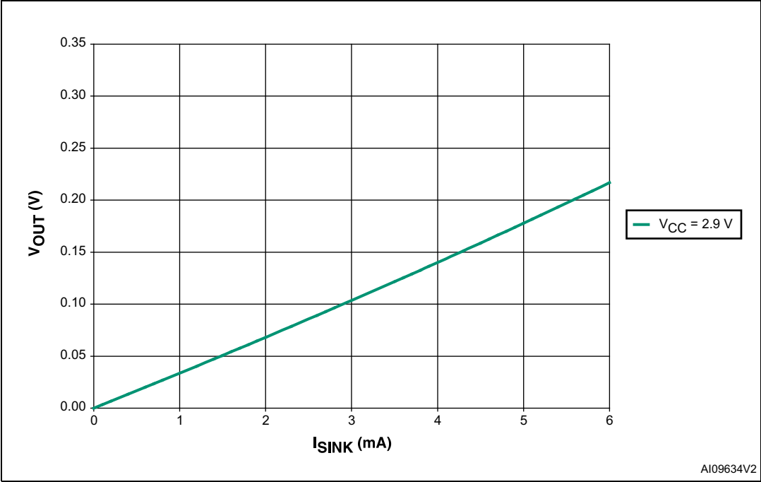
Figure 21. Voltage output low vs. I_{SINK}
