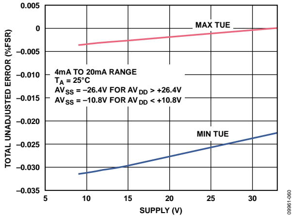
Figure 43. Total Unadjusted Error vs. Supply, External R SET
