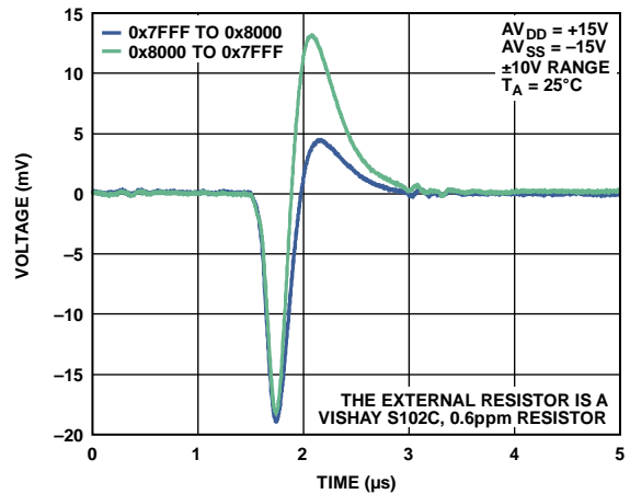
Figure 25. Digital-to-Analog Glitch
