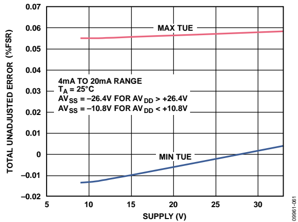
Figure 44. Total Unadjusted Error vs. Supply, Internal R SET
