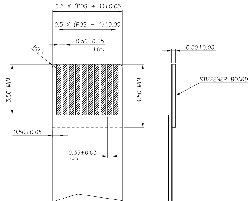
RECOMMENDED FPC DIMENSIONS DIAGRAM TOLERANCE \pm 0.05
