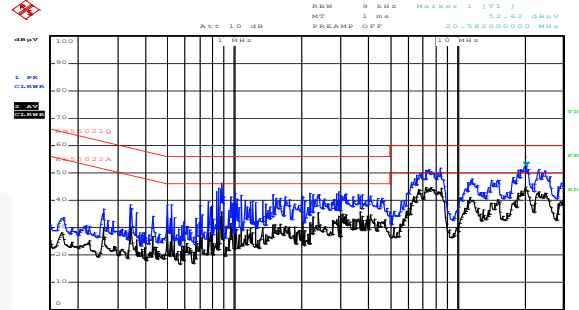
Figure 57. Neutral: 230 V AC / 50 Hz & 9 V O
