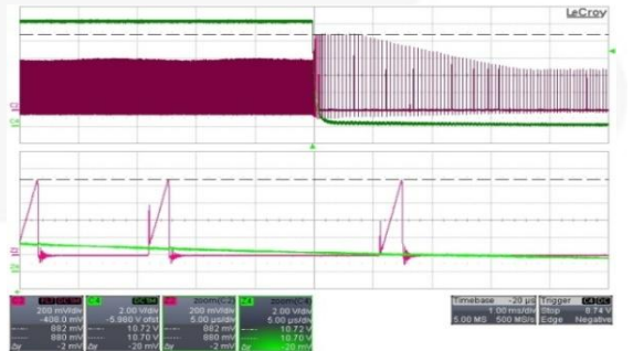
Figure 30. C2[V Cs ], C4[V O ], 264 V AC /50 Hz, I O =1.25 A, V O =12 V
