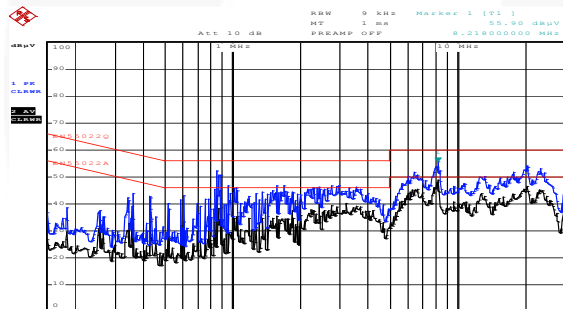
Figure 58. Line: 115 V AC / 60 Hz & 12 V O
