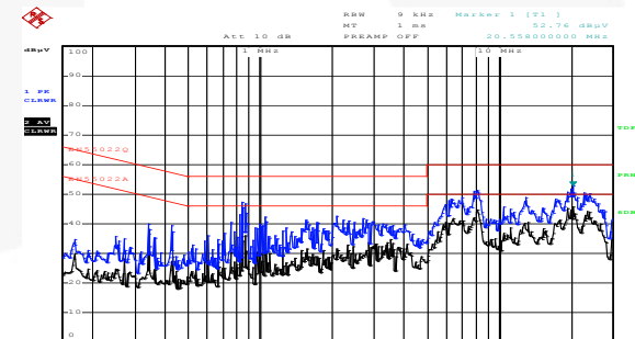
Figure 59. Neutral: 115 V AC / 60 Hz & 12 V O
