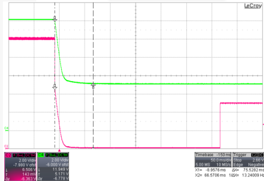
Figure 48. C2[V BLD ], C4[V O ] 90 V AC / 60 Hz & I O =0 A, 12 V to 5 V
