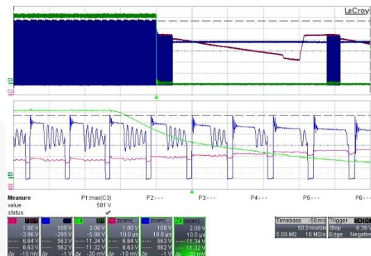
Figure 34. C2[FB], C3[V bs ], C4[Vo] 264 V AC /50 Hz, 12 V, Full Load Output Short
