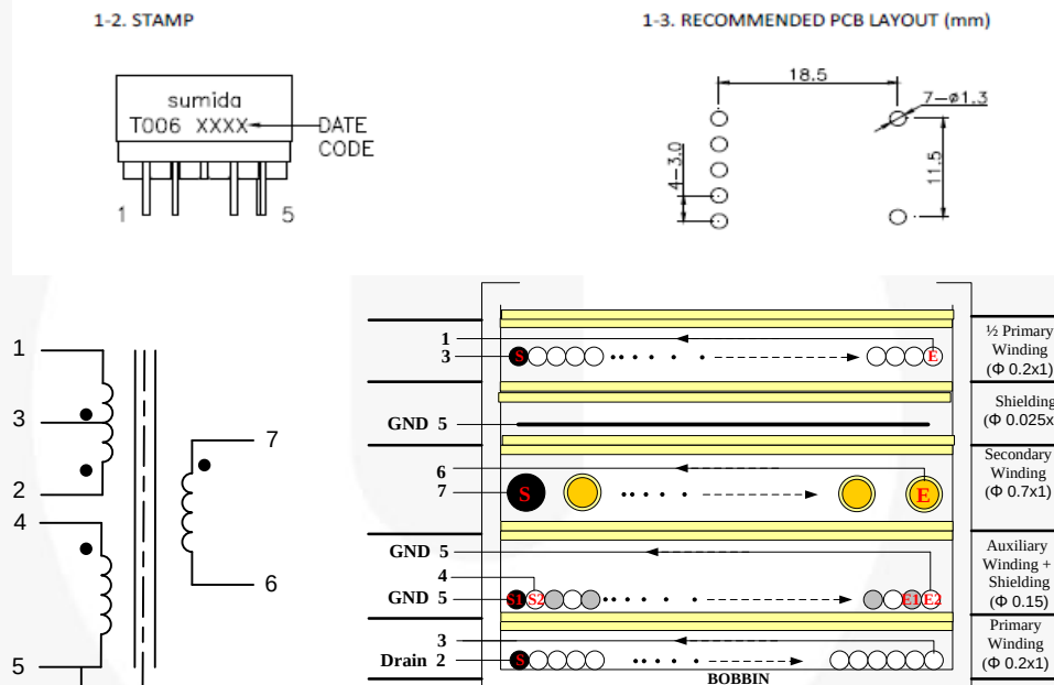
Figure 7. Transformer Specifications & Construction
