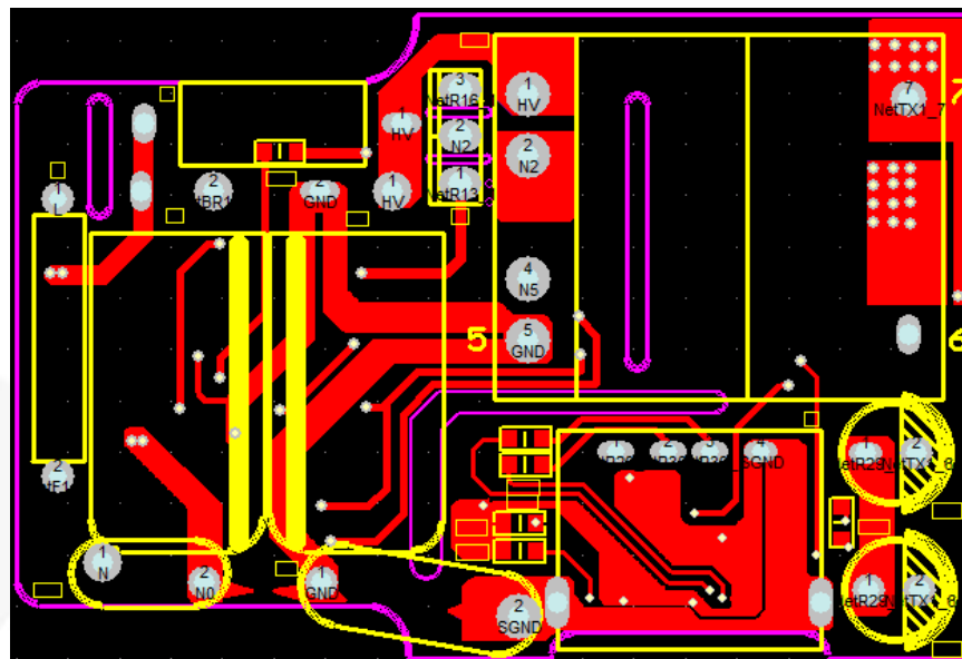
Figure 4. Top View
