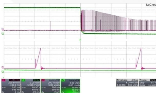
Figure 29. C2[V_{CS}] , C4[V_O] , 264 V AC /50 Hz, I O =0 A, V O =12 V
