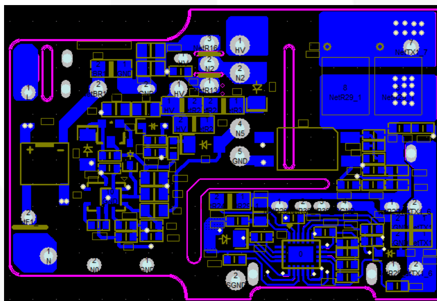
Figure 5. Bottom View
