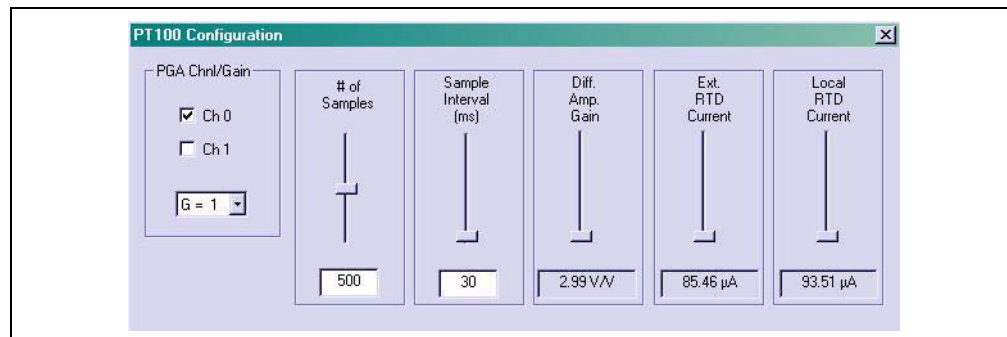
FIGURE 2-6: Hardware Status
