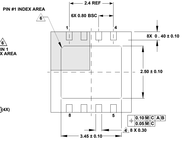
BOTTOM VIEW
