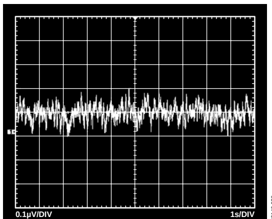
Figure 29. 0.1 Hz to 10 Hz RTI Voltage Noise ( G = 1000 )
