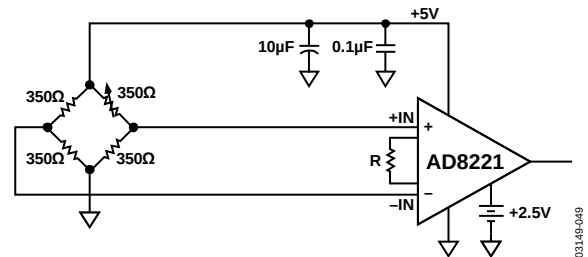
Figure 50. Precision Strain Gage
