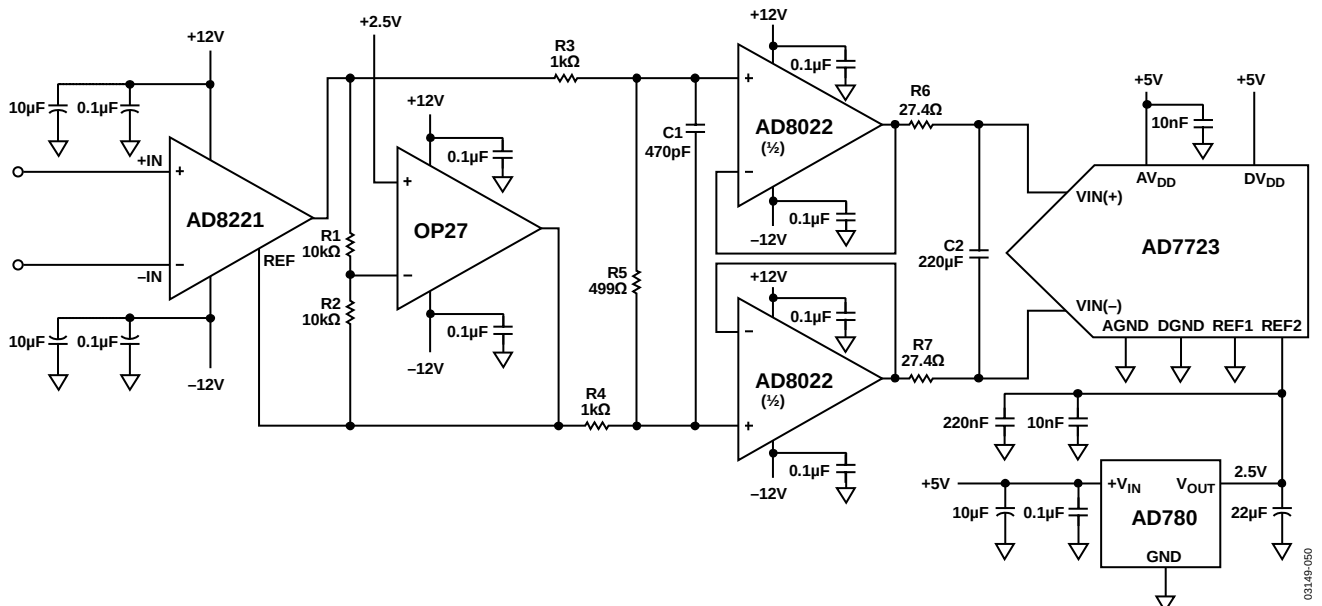
Figure 51. Interfacing to a Differential Input ADC
