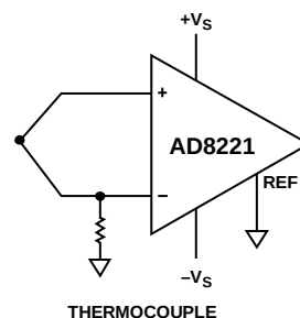
THERMOCOUPLE
