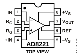
Figure 44. Pinout Diagram
