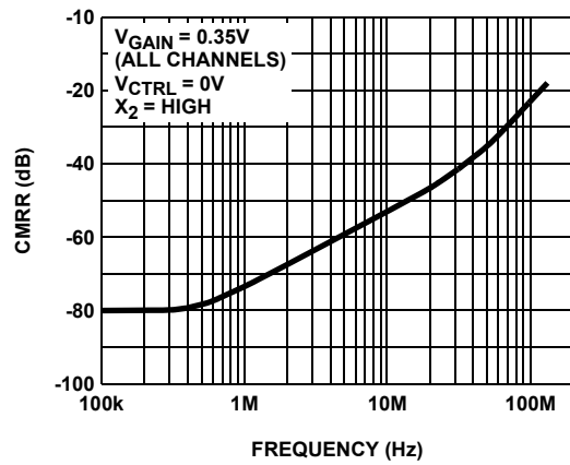
FIGURE 11. COMMON-MODE REJECTION
