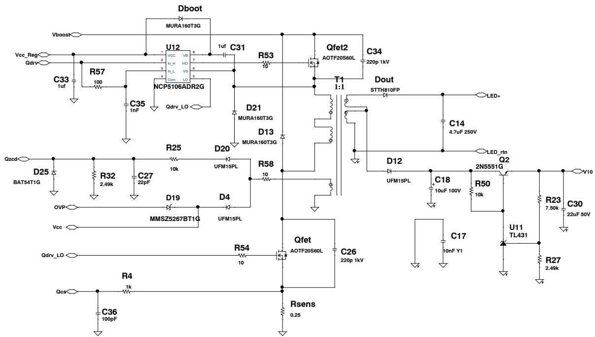
Figure 6. Flyback Schematic
