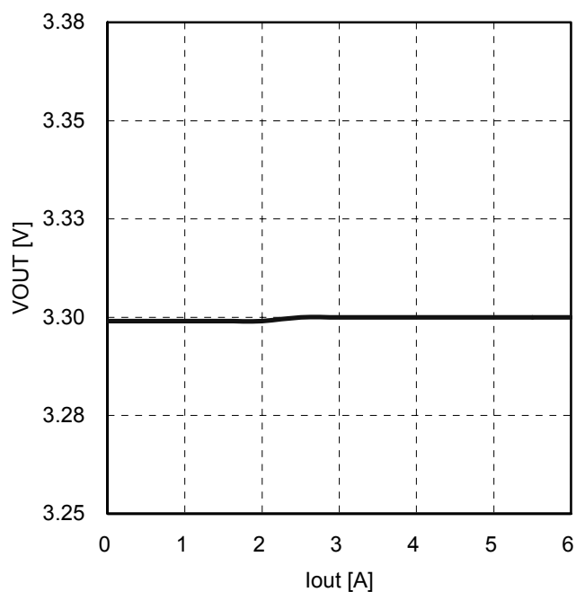
Figure.8 VOUT Load Regulation ( V_{\text{IN}}=12\text{V} , V_{\text{OUT}}=3.3\text{V} , L=2.2\mu\text{H} )
