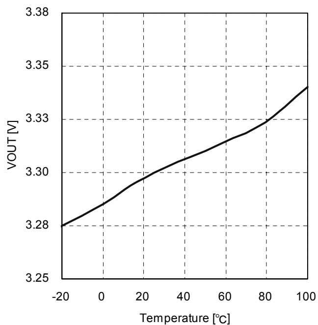
Figure.10 VOUT - Temperature ( V_{\text{IN}}=12\text{V} , V_{\text{OUT}}=3.3\text{V} , L=2.2\mu\text{H} , I_{\text{out}}=0\text{A} )
