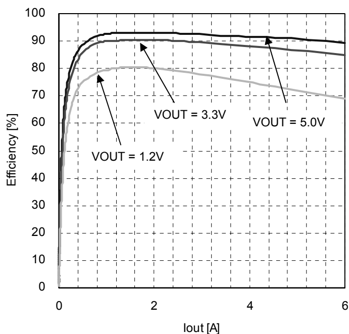
Figure.4 Efficiency ( V_{\text{IN}}=12\text{V} , L=2.2\mu\text{H} )
