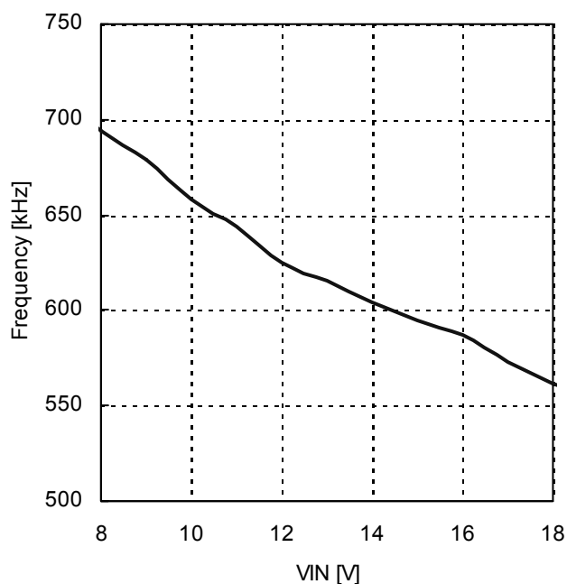
Figure.11 Frequency - VIN ( V_{\text{IN}}=12\text{V} , V_{\text{OUT}}=3.3\text{V} , L=2.2\mu\text{H} , I_{\text{out}}=0\text{A} )
