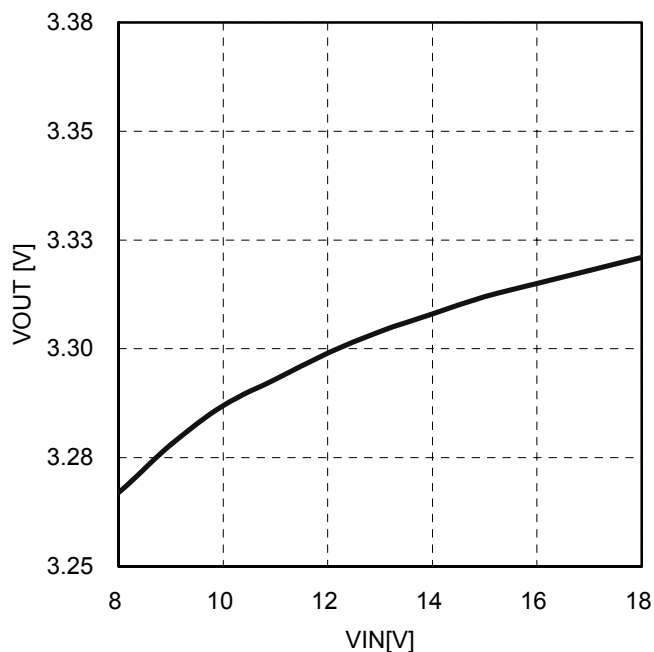
Figure.9 VOUT Line Regulation ( V_{\text{OUT}}=3.3\text{V} , L=2.2\mu\text{H} , I_{\text{out}}=0\text{A} )
