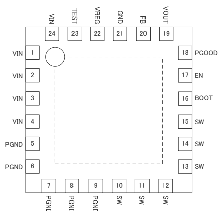
Figure.2 Pin Configuration
