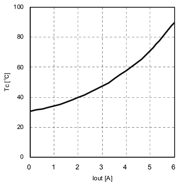
Figure.5 T_c - I_{\text{out}} ( V_{\text{IN}}=12\text{V} , V_{\text{OUT}}=3.3\text{V} , L=2.2\mu\text{H} )
