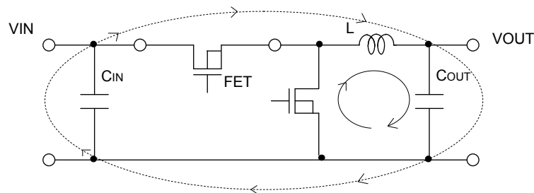
Figure.27 Current loop Buck regulator system
