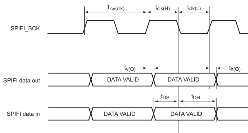
Fig 39. SPIFI timing
