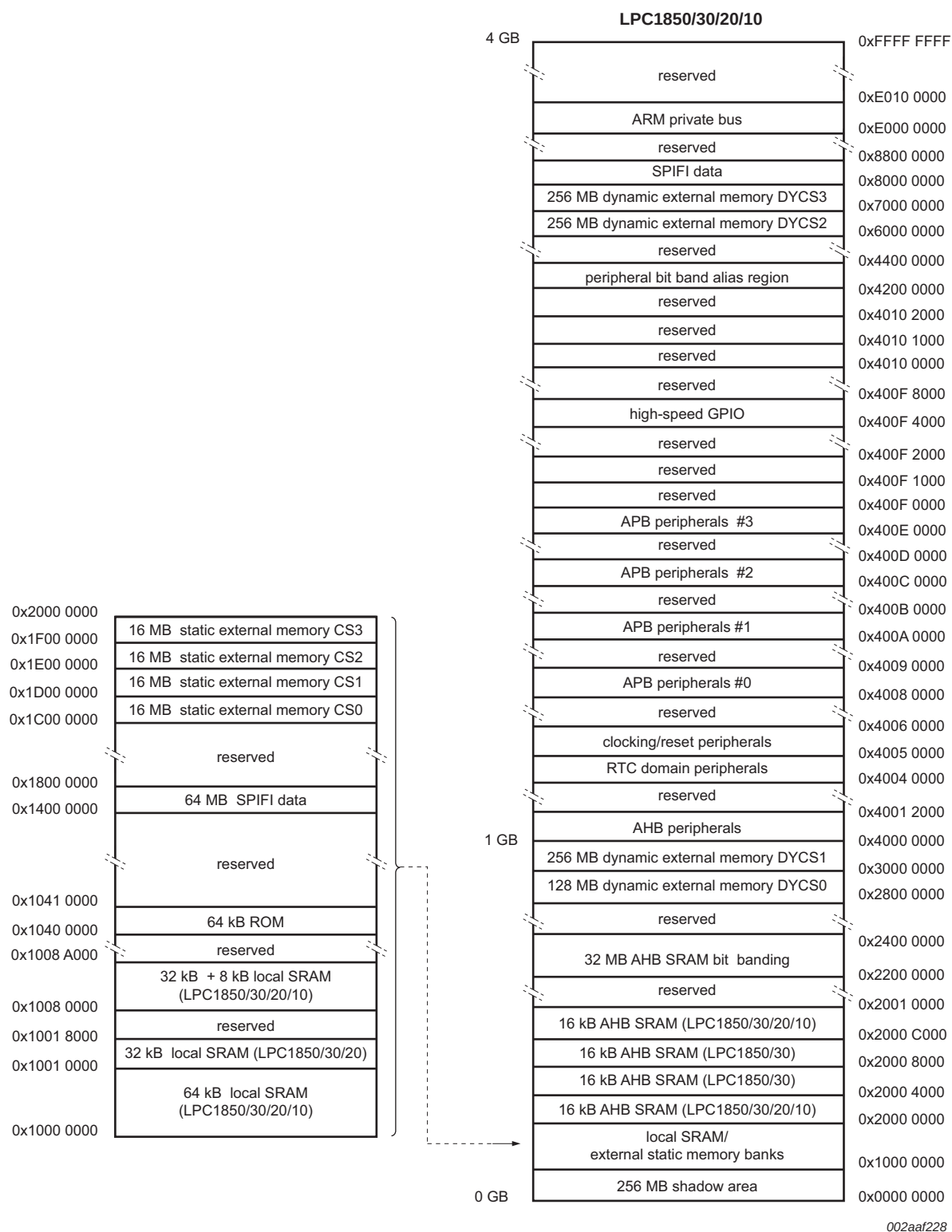
Fig 8. LPC1850/30/20/10 Memory mapping (overview)
