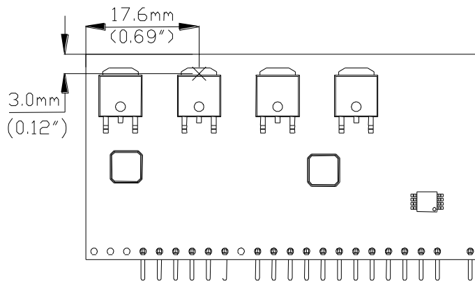
Figure 41: Temperature measurement location * The allowed maximum hot spot temperature is defined at 125 °C
