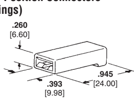
A — Receptacle Housing
