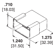
Tab Housing
