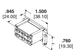
Receptacle Housing
