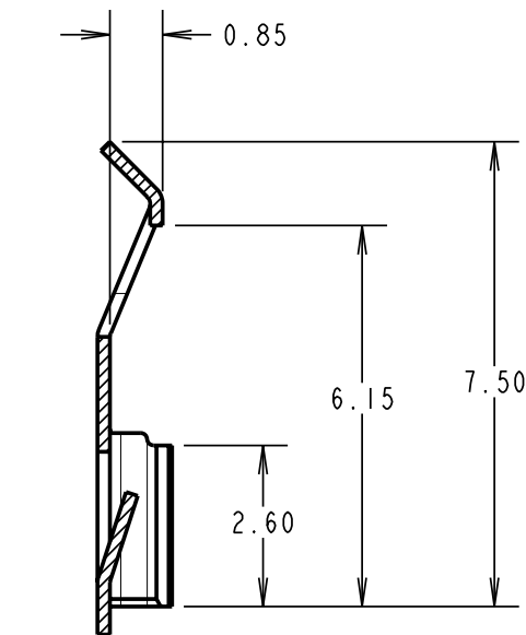
SECTION X-X
