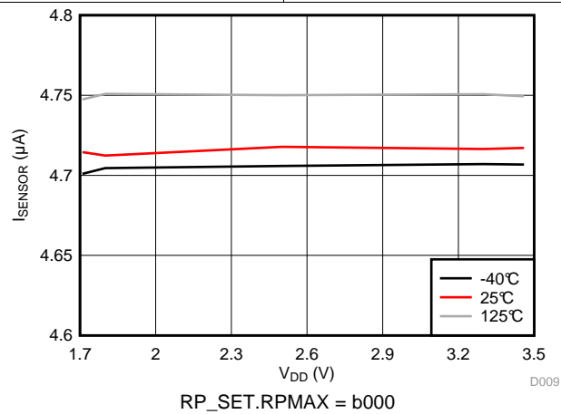
Figure 11. I_{SENSOR-MIN} vs V_{DD}
