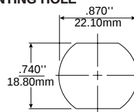
Knockout Hole
