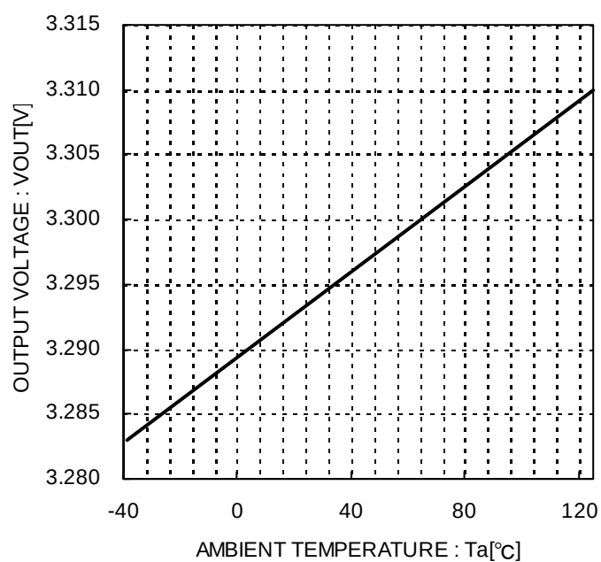
Figure 13. Output voltage vs. temperature
