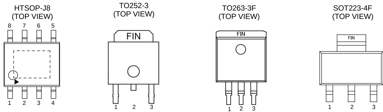
Figure 3. Pin Configuration
