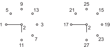
19 Rotary selector switching element 45° page 53
