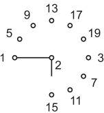
15 Rotary selector switching element 30° page 53
