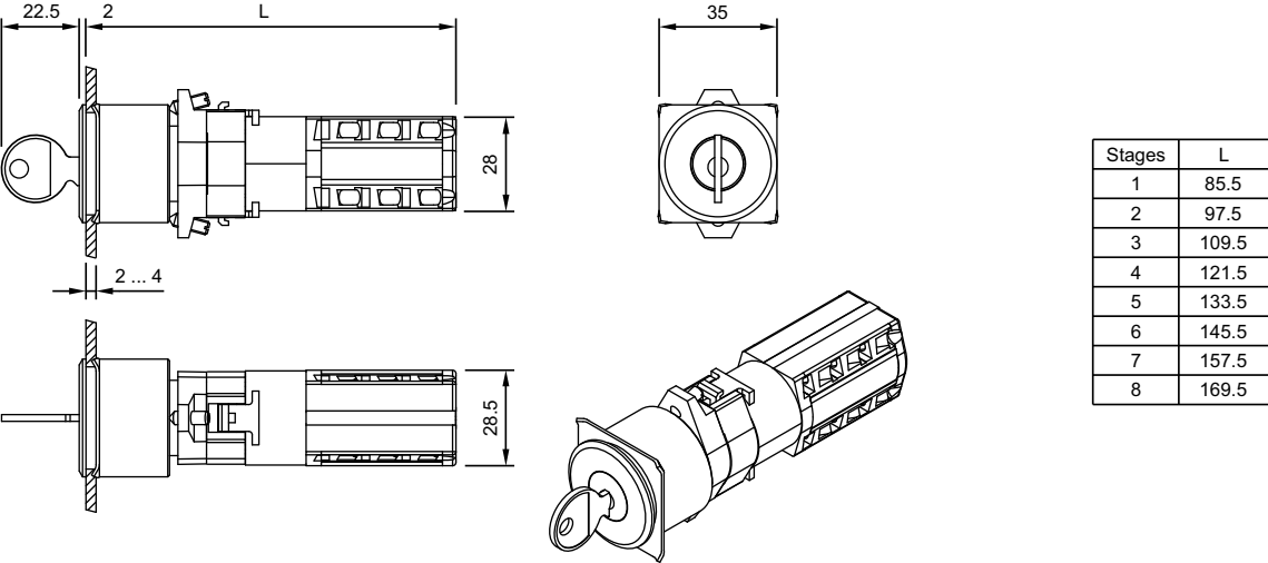
68 Keylock rotary switch actuator, flush mounting page 44
