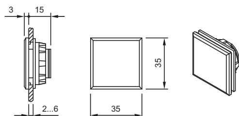
43 Blind plug page 48
