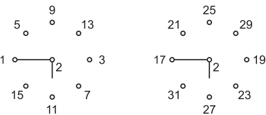
20 Rotary selector switching element 45° page 53
