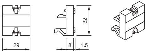
37 Snap-on base page 59
