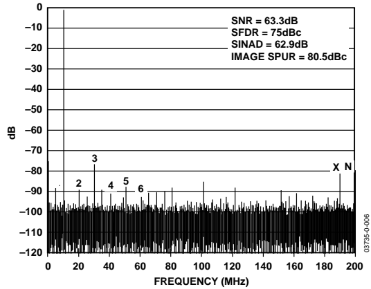
Figure 6. FFT: f_s = 400 MSPS, A_{IN} = 10.123 MHz @ -1.0 dBFS
