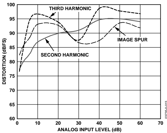
Figure 14. 2nd/3rd Harmonics and Image Spur vs. Analog Input Level— f_s = 400 MSPS, A_{IN} = 70 MHz
