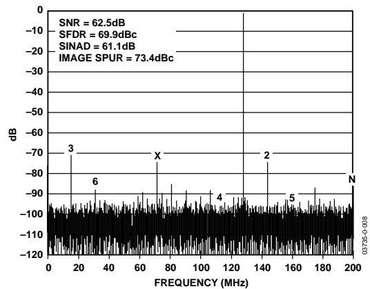
Figure 8. FFT: f_s = 400 MSPS, A_{IN} = 128.123 MHz @ -1.0 dBFS
