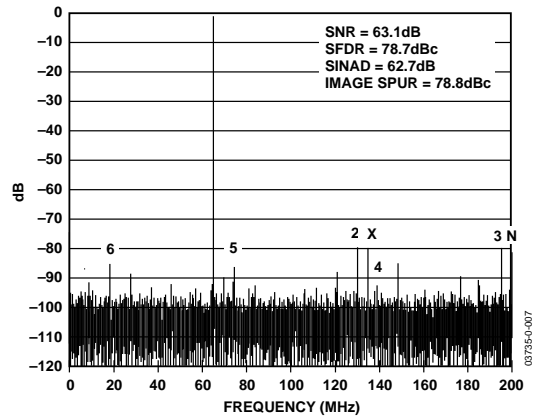
Figure 7. FFT: f_s = 400 MSPS, A_{IN} = 65.123 MHz @ -1.0 dBFS
