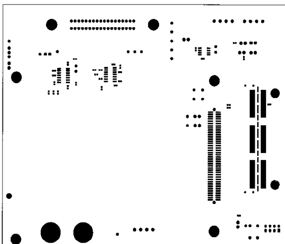
Figure 31. Top Mask
