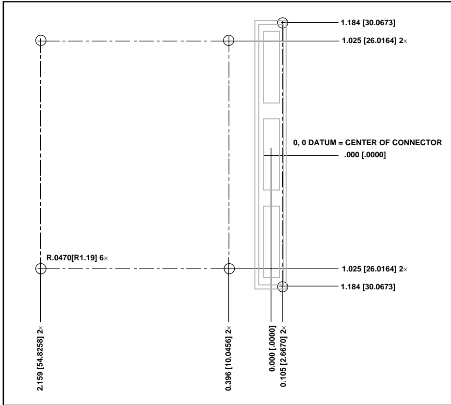
Figure 37. Top View of Interface PCB Assembly
