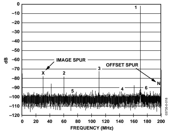
Figure 19. AD12400 with AFB Digital Post Processing
