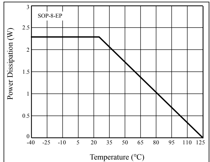
Figure 35 Dissipation Curve
