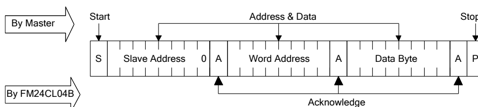
Figure 5. Byte Write
