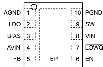
3mm x 3mm MLF-10L (ML)
