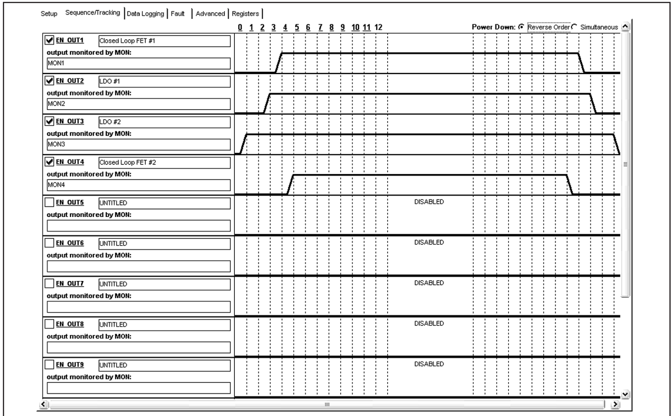
Figure 4. Sequence/Tracking Tab
