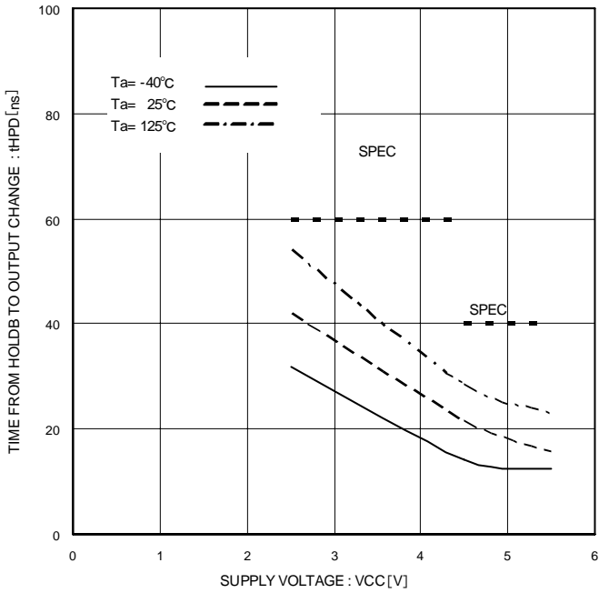
Figure 31. Time from HOLD to Output Change tHPD
