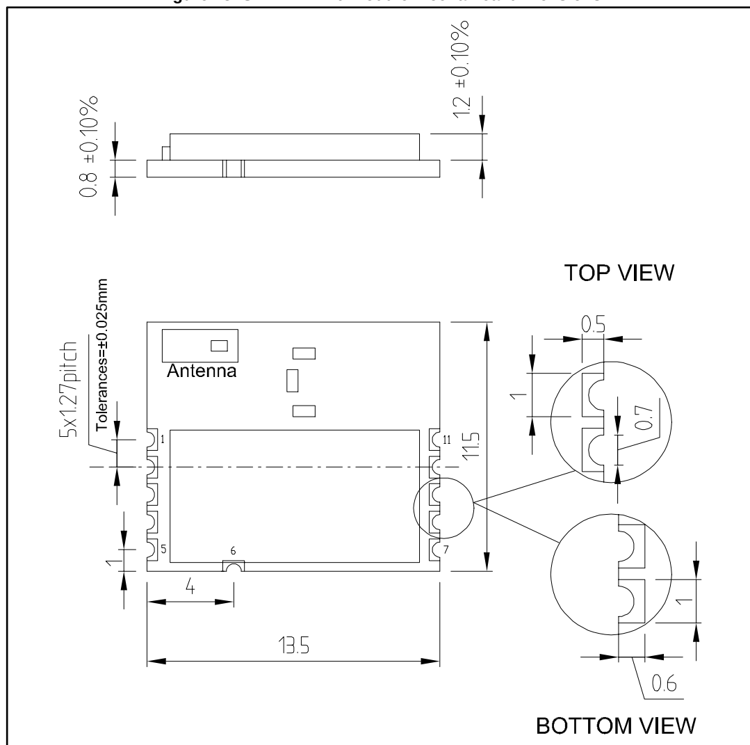
Figure 13: SPBTLE-RF0 module mechanical dimensions
