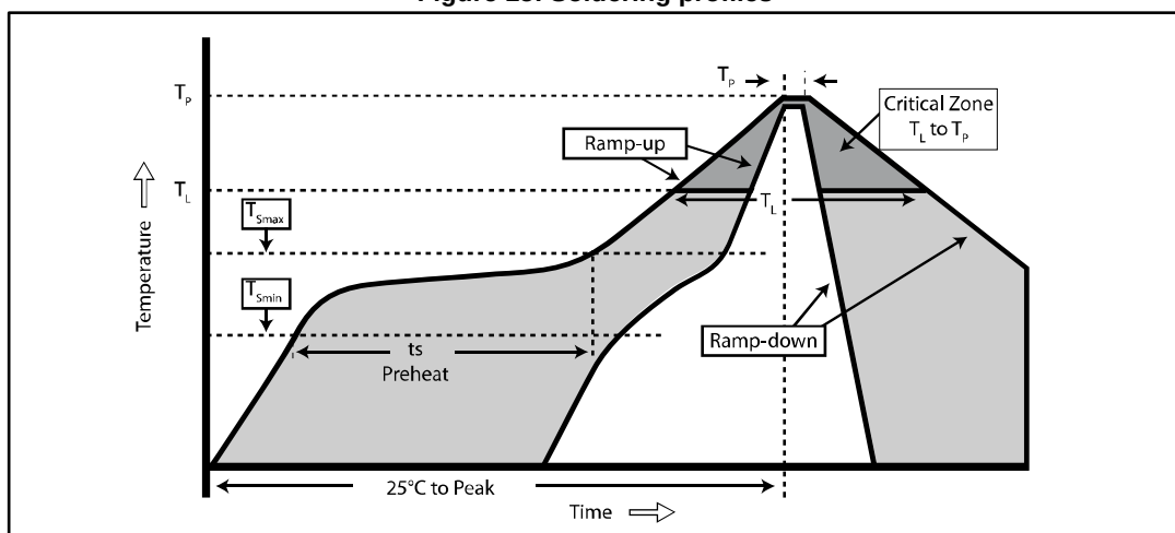
Figure 15: Soldering profiles
