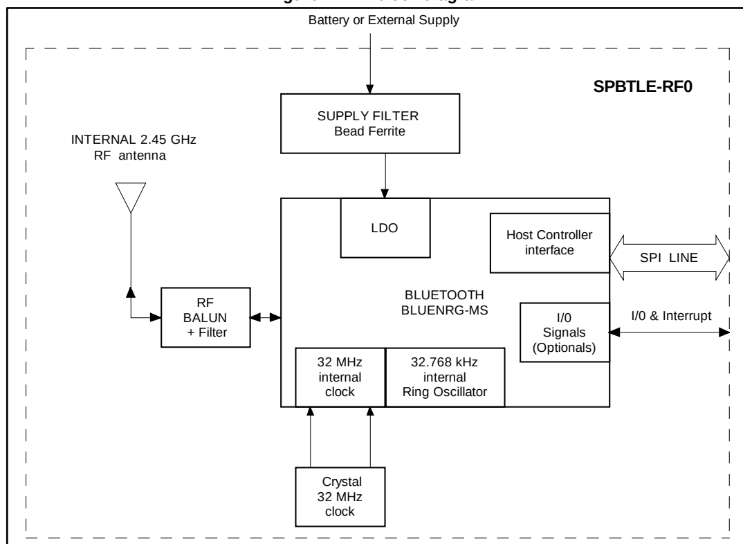
Figure 1: HW block diagram
