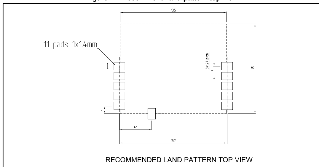
Figure 14: Recommend land pattern top view
