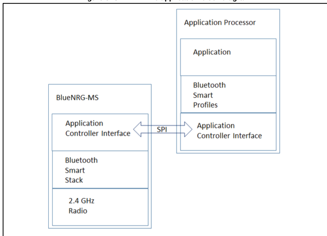
Figure 3: SPBTLE-RF0 application block diagram
