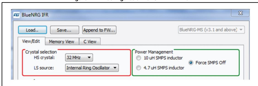
Figure 2: IFR configuration for SPBTLE-RF0
