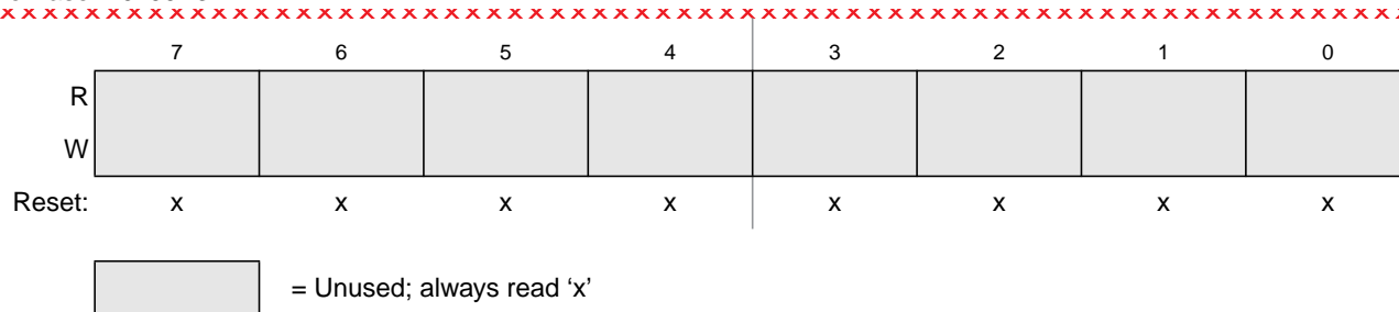
Figure 8-33. Identifier Register 3 — Standard Mapping
