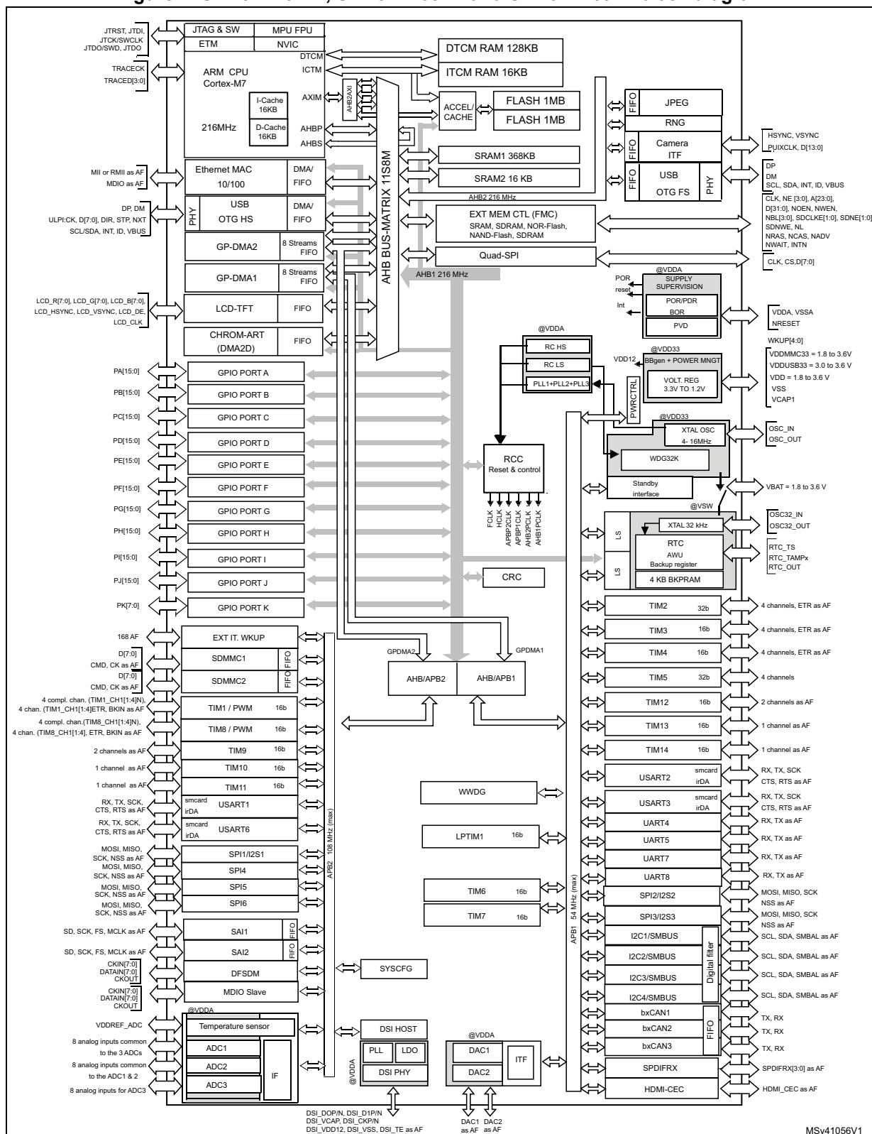
Figure 2. STM32F767xx, STM32F768Ax and STM32F769xx block diagram
