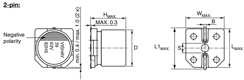
Fig. 2 - Dimensional outline
