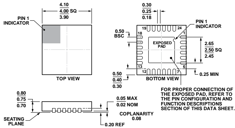
Figure 60. 24-Lead Lead Frame Chip Scale Package [LFCSP_WQ] 4 mm × 4 mm Body, Very Thin Quad (CP-24-7) Dimensions shown in millimeters
