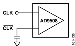
Figure 37. Typical 1.8 V CMOS Configurations for Short Trace Lengths
