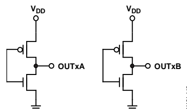
Figure 44. CMOS Equivalent Output Circuit
