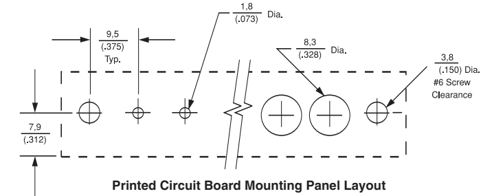
Printed Circuit Board Mounting Panel Layout
