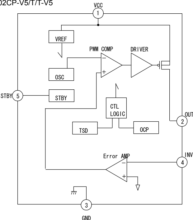
Fig.28 Block Diagram
