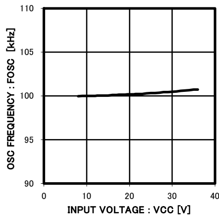
Fig.8 fosc-INPUT VOLTAGE
