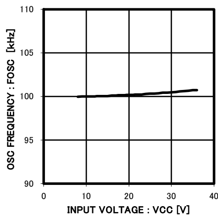
Fig.8 fosc-INPUT VOLTAGE
