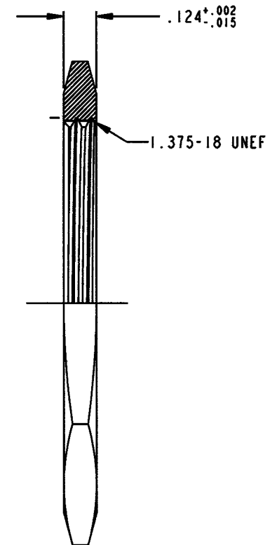
SECTION Z-Z
