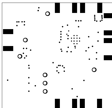
Figure 6-7. Bottom Solder
