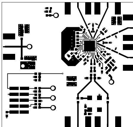
Figure 6-3. Top Layer
