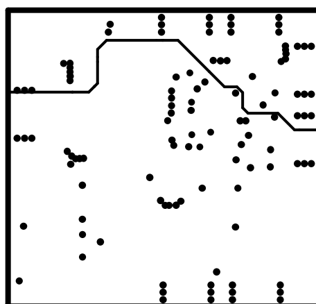
Figure 6-5. Power Layer
