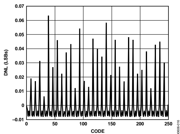
Figure 15. Typical DNL
