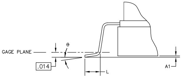
DETAIL "G"
