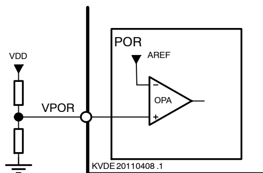
Figure 13. Power on Reset Block
