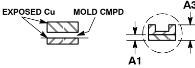
DETAIL B OPTIONAL CONSTRUCTIONS
