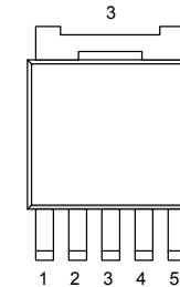
NJW4188DL3 TO252-5
