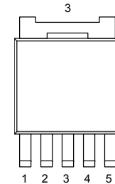
NJW4187DL3 TO252-5
