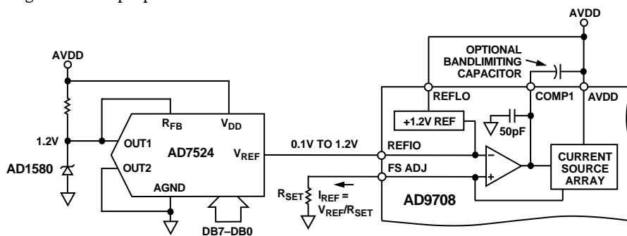
Figure 15. Single-Supply Gain Control Circuit
