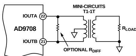
Figure 23. Differential Output Using a Transformer
