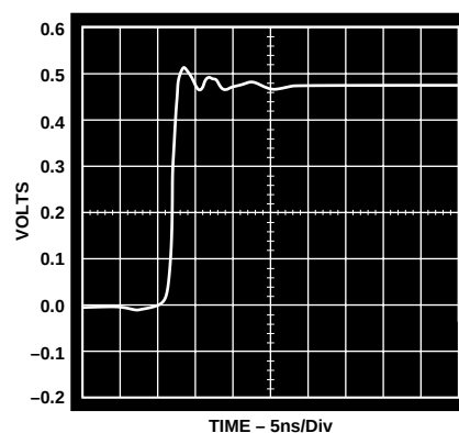
Figure 11. Step Response
