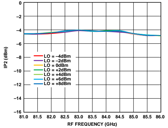
Figure 33. Input IP2 vs. RF Frequency at Various LO Powers, I_{FIN} = 5 \text{ dBm} , IF = 1000 \text{ MHz} , USB
