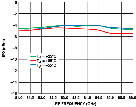
Figure 30. Input IP2 vs. RF Frequency at Various Temperatures, I_{FIN} = 5 \text{ dBm} , LO = 2 \text{ dBm} , IF = 1000 \text{ MHz} , USB
