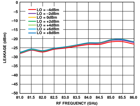
Figure 34. 6 \times LO Leakage at RFOUT vs. RF Frequency at Various LO Powers, I_{FIN} = 5 \text{ dBm} , IF = 1000 \text{ MHz} , USB
