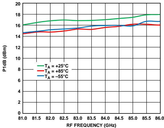
Figure 32. Input P1dB vs. RF Frequency at Various Temperatures, LO = 2 \text{ dBm} , IF = 1000 \text{ MHz} , USB
