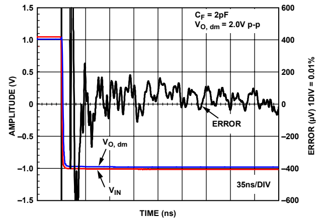
Figure 36. Settling Time (0.01%)
