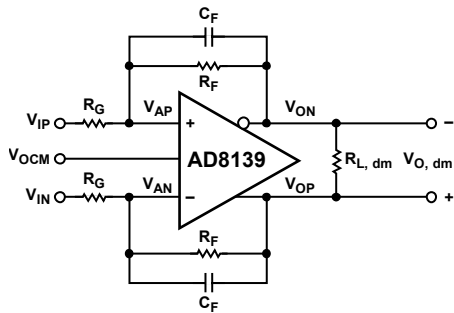
Figure 59. Typical Connection
