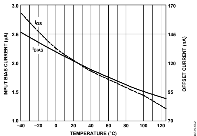
Figure 49. Input Bias and Offset Current vs. Temperature
