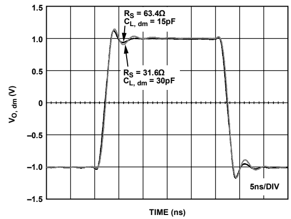
Figure 35. Large Signal Transient Response for Capacitive Loads
