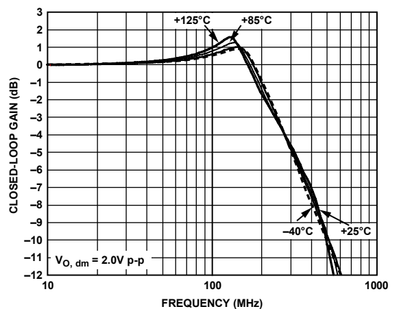
Figure 12. Large Signal Frequency Response at Various Temperatures
