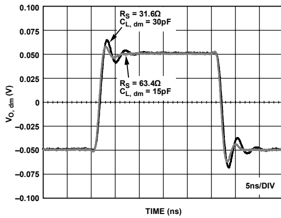
Figure 32. Small Signal Transient Response for Capacitive Loads
