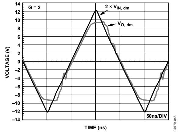
Figure 46. Overdrive Recovery
