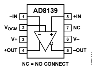
Figure 1. 8-Lead SOIC
