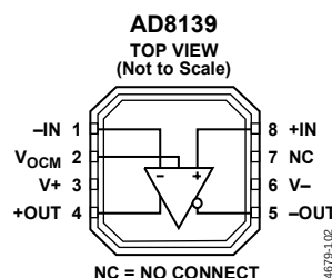
Figure 2. 8-Lead LFCSP
