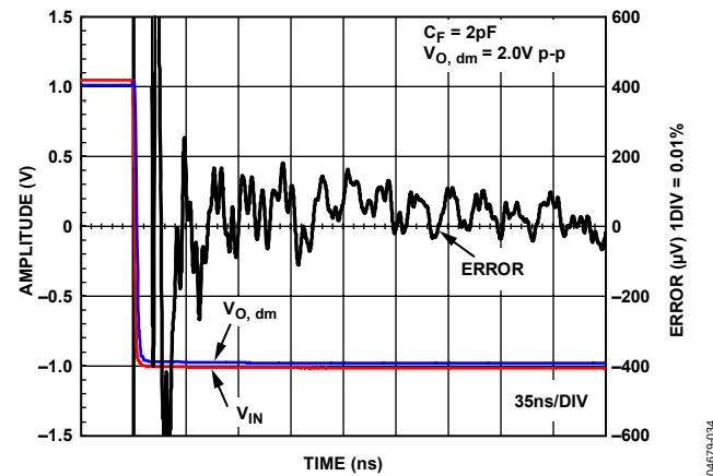
Figure 36. Settling Time (0.01%)
