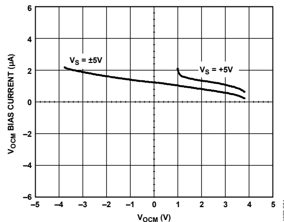
Figure 56. V_{OCM} Bias Current vs. V_{OCM} Input Voltage
