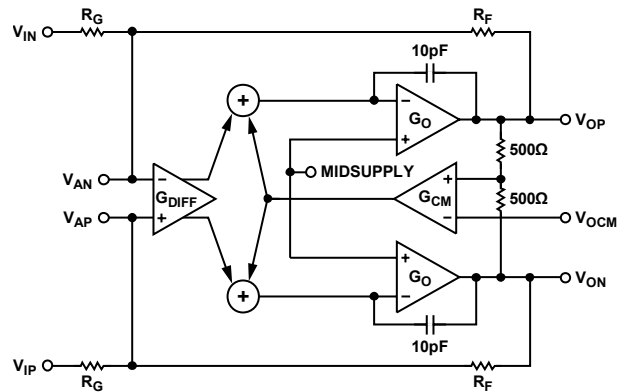
Figure 60. Block Diagram
