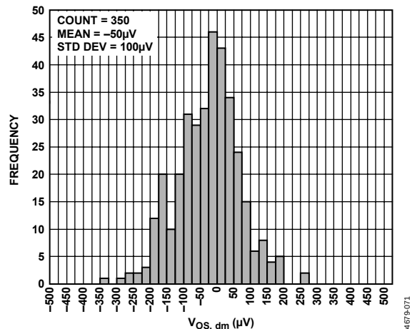
Figure 54. V_{OS, dm} Distribution
